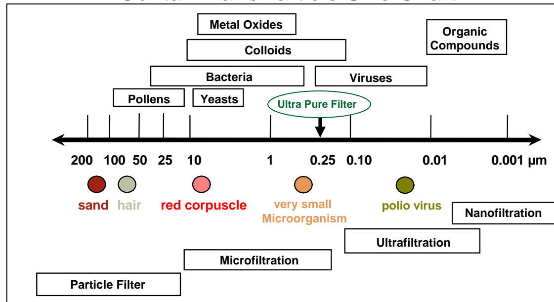
Contaminant/Particle Size Chart
